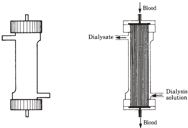
Hollow-fiber dialyzer
